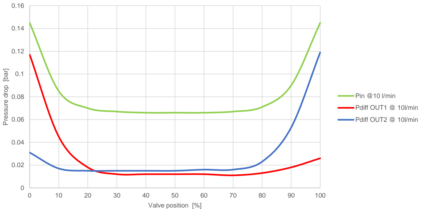
Pressure drop @ 10l/min
